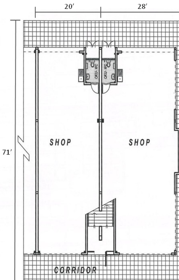
Floor Plan
